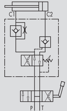
SCHEMA IDRAULICO HYDRAULIC DIAGRAM
